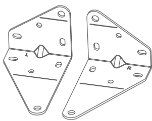
Pillar Fixing Bracket (x2)
